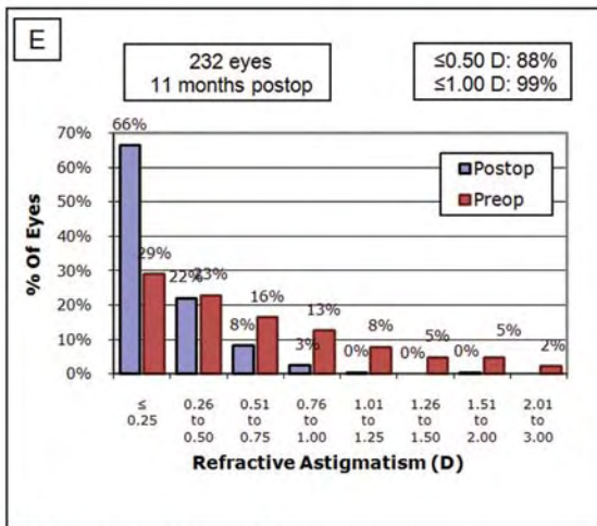
Refractive Astigmatism
